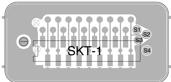
220-01383-01 TOP COPPER/DEVICES
