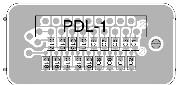
220-01383-01 BOTTOM COPPER/DEVICES
